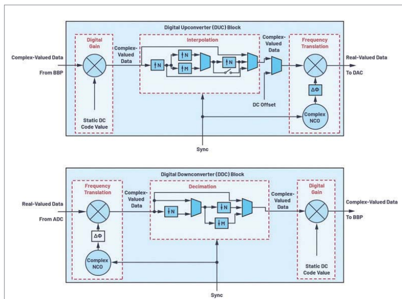
2. DUC and DDC blocks provide many useful DSP features now within converter ICs.
