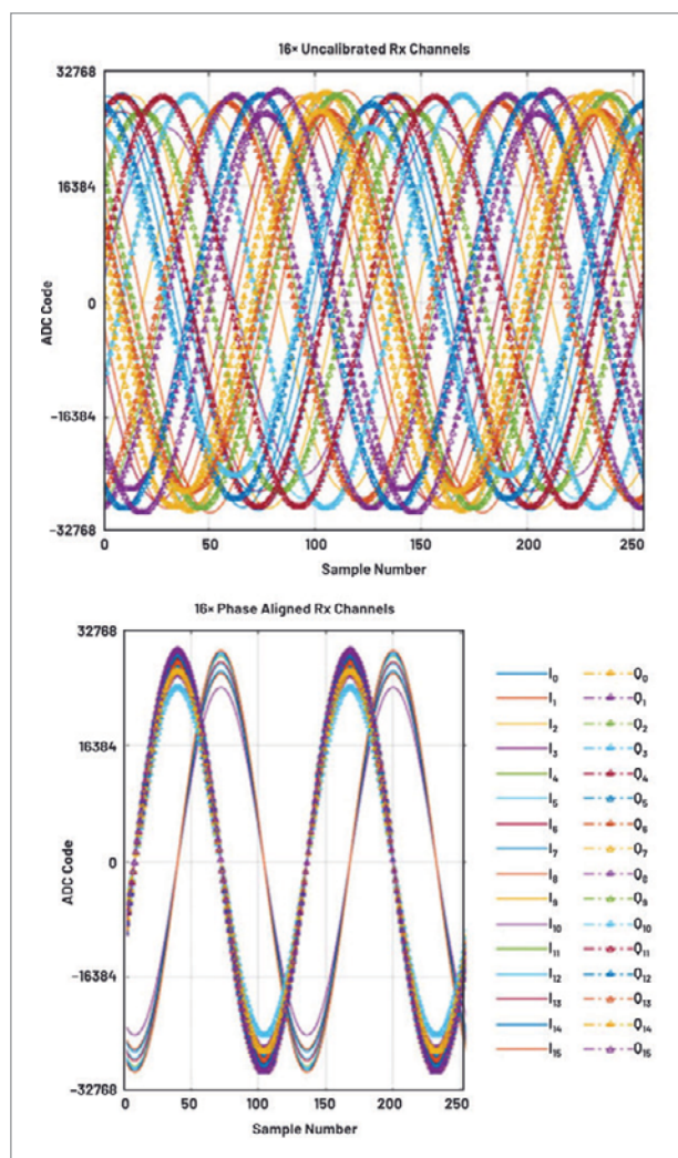
3. Experimental results showing the simultaneous I/Q capture of 16 receive channels that are phase aligned (but not amplitude aligned) strictly using the complex NCO phase offsets provided in DDC blocks located on the digitizer IC.
