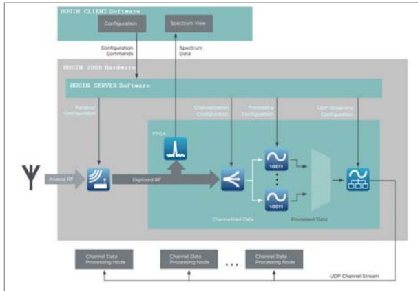
9. Novator Solutions's updated HUGIN 2000 receivers deliver improved signal quality, more flexibility/usability, and greater up-time for COMINT applications.
