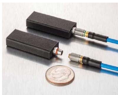
5. TLMP push-on connectors are sized like SMP connectors, but offer many performance advances to serve the operating environments of military UAVs. (Courtesy of Times Microwave Systems)
